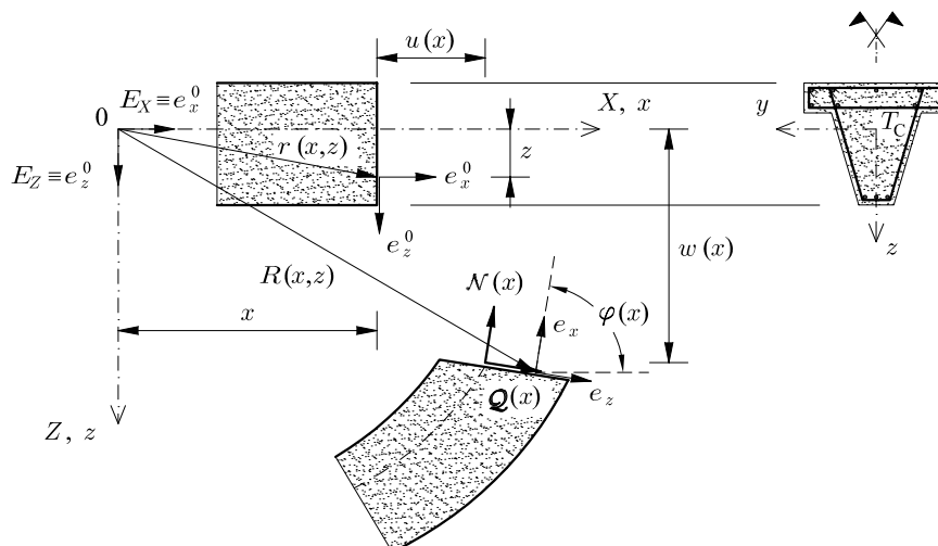
Figure 1: Deformed and undeformed configurations of the beam.
