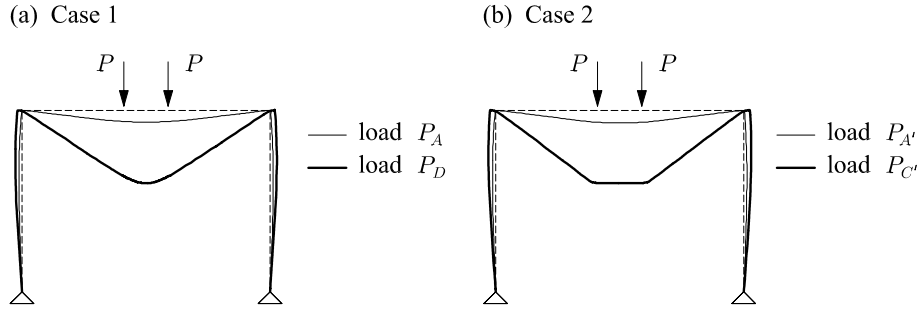
Figure 18. Cranston's portal frame. The comparison of deformed shapes in the softening phase (magnified 15\times ).
