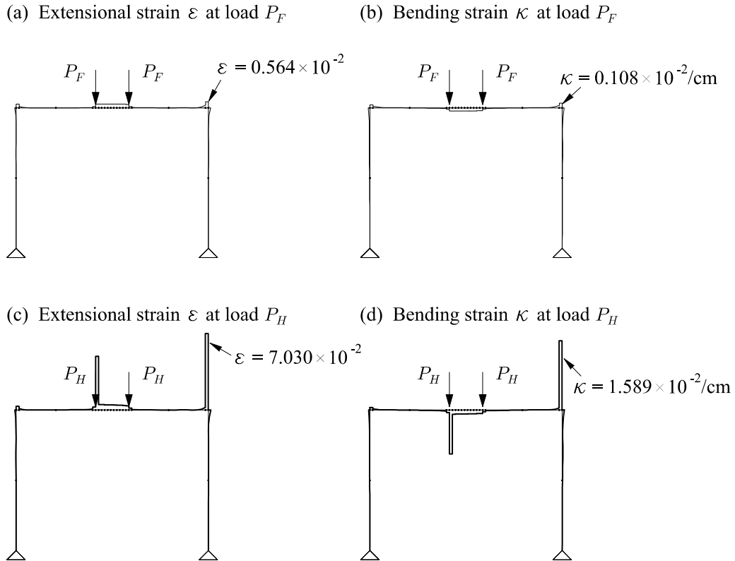
Figure 21. Cranston's portal frame with the geometric imperfection. The distribution of strain measures, \varepsilon and \kappa , along the axis of the frame. (a) \varepsilon at P_F , (b) \kappa at P_F , (c) \varepsilon at P_H , (d) \kappa at P_H .
