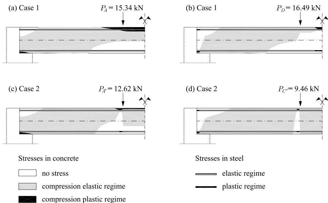
Figure 16. Cranston’s portal frame. Stresses in the beam. (a) At load P_A = 15.34 \text{ kN} (point A ); (b) at load P_D = 16.49 \text{ kN} (point D ); (c) at load P_{A'} = 12.62 \text{ kN} (point A' ); (d) at load P_{C'} = 9.46 \text{ kN} (point C' ).
