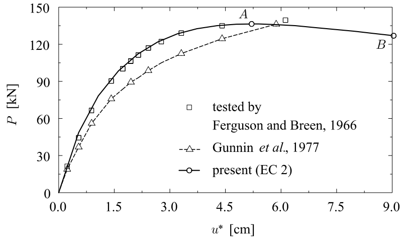
Figure 9. Square frame. Load vs horizontal deflection curve.
