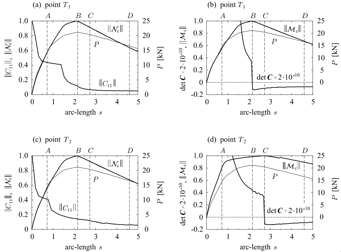
Figure 14. Cranston's portal frame. Graphs of \mathcal{N}_c , \mathcal{M}_c , \mathcal{C}_{11} , and \det \mathbf{C} , as functions of arc-length s . (a)–(b) At the left-end cross-section of the beam, point T_1 , (c)–(d) at the mid-point cross-section of the beam, point T_2 .
