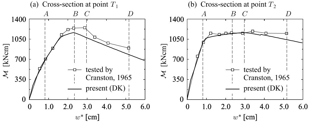
Figure 15. Cranston's portal frame. Bending moments. (a) At the left-end cross-section of the beam, point T_1 , (b) at the mid-point cross-section of the beam, point T_2 .
