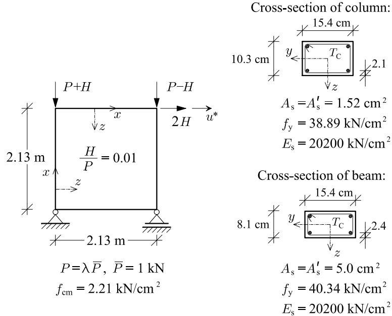
Figure 8. Square frame of Ferguson and Breen (1966). Geometric, material, and loading data.
