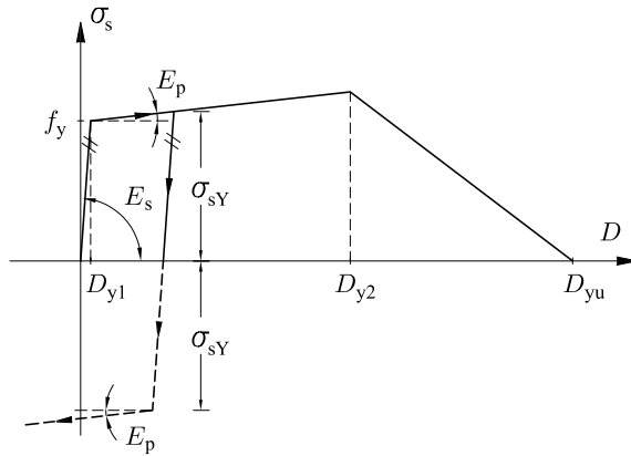
Figure 3: Constitutive law of reinforcing steel.
