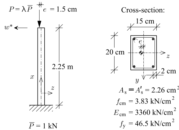
Figure 5: Foue's column. Geometric, material, and loading data.
