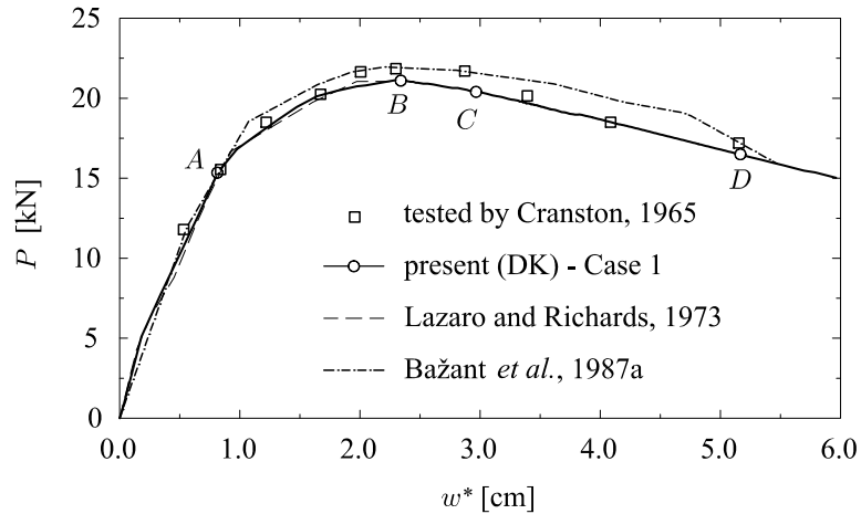
Figure 13. Cranston's portal frame. Load-mid-point deflection curves.
