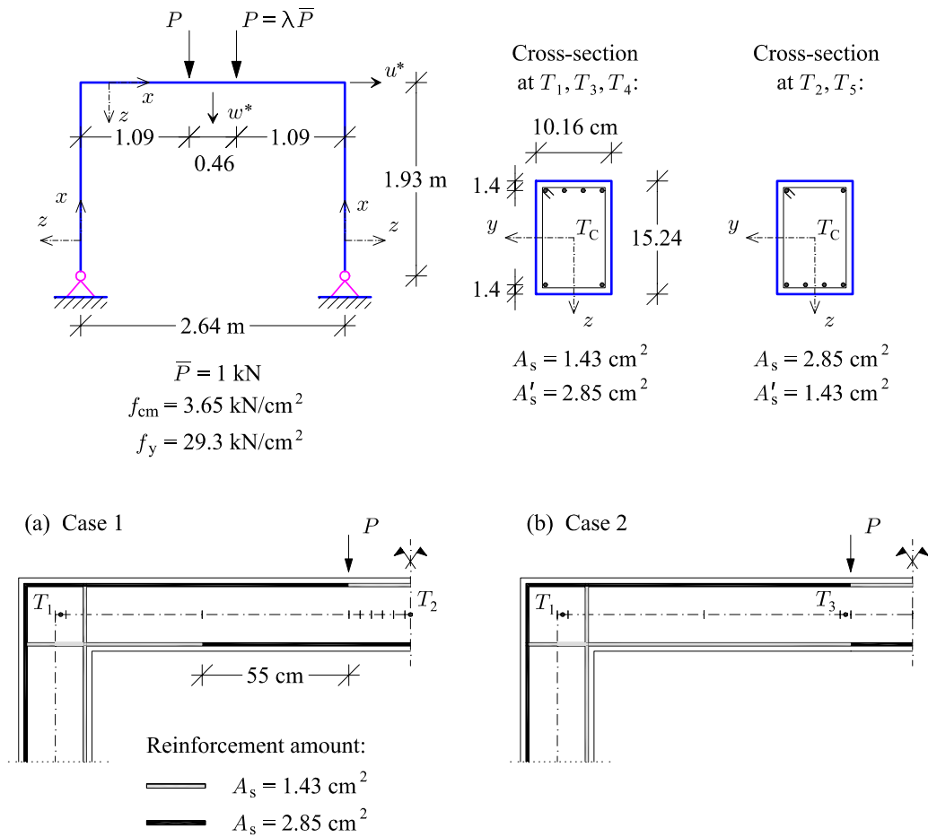
Figure 12. Cranston's portal frame. Geometrical, material, and loading data. (a) Original position of reinforcement (Case 1); (b) alternative position of reinforcement (Case 2).
