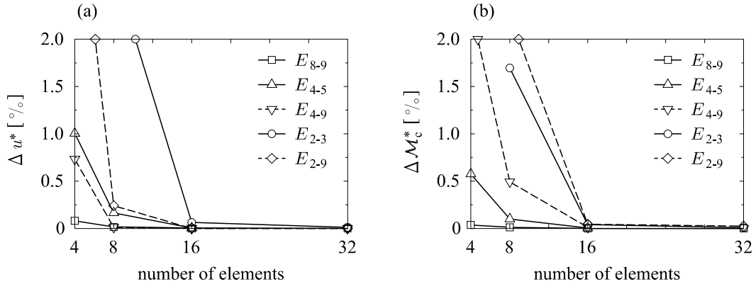
Figure 10. Square frame. The accuracy of results as a function of number and type of finite elements at load P = 130 \text{ kN} . (a) Horizontal displacement, \Delta u^* = \left| \frac{u^* - u_{32}^*}{u_{32}^*} \right| ; (b) constitutive moment at the top of the right-hand column, \Delta \mathcal{M}_c^* = \left| \frac{\mathcal{M}_c^* - \mathcal{M}_{c,32}^*}{\mathcal{M}_{c,32}^*} \right| .
