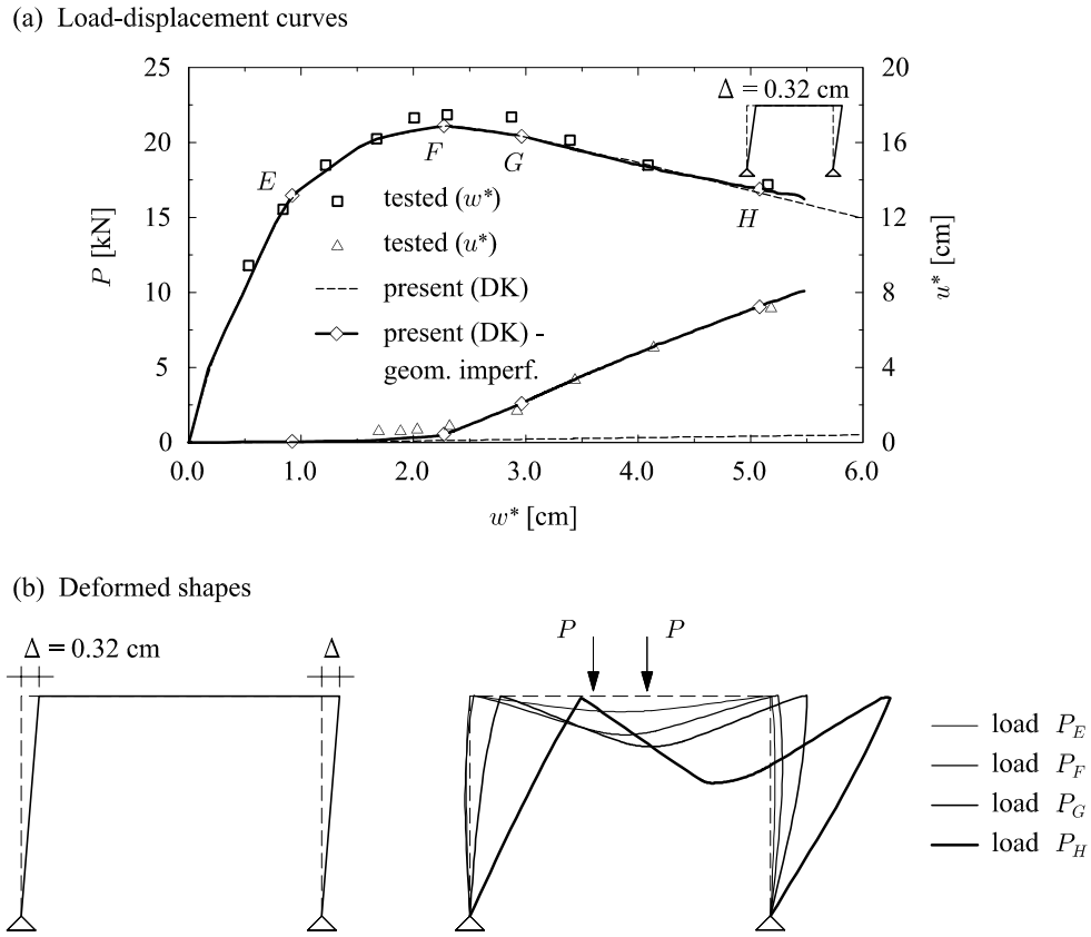
Figure 20. Cranston's portal frame with the geometric imperfection. (a) Load-displacement curves; (b) deformed shapes in softening regime ( 15\times magnified).
