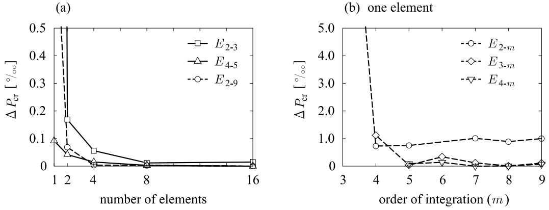
Figure 7. Foure's column. The error of P_{cr} vs (a) number of finite elements, (b) order of numerical integration; \Delta P_{cr} = \left| \frac{P_{cr} - P_{cr,16}}{P_{cr,16}} \right| .
