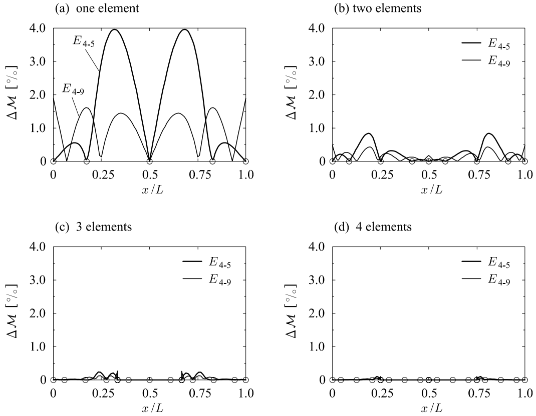
Figure 11. Square frame. The graph of \Delta\mathcal{M} = \left| \frac{\mathcal{M}_c - \mathcal{M}}{\mathcal{M}_{\max}} \right| vs x/L for the right-hand column.
