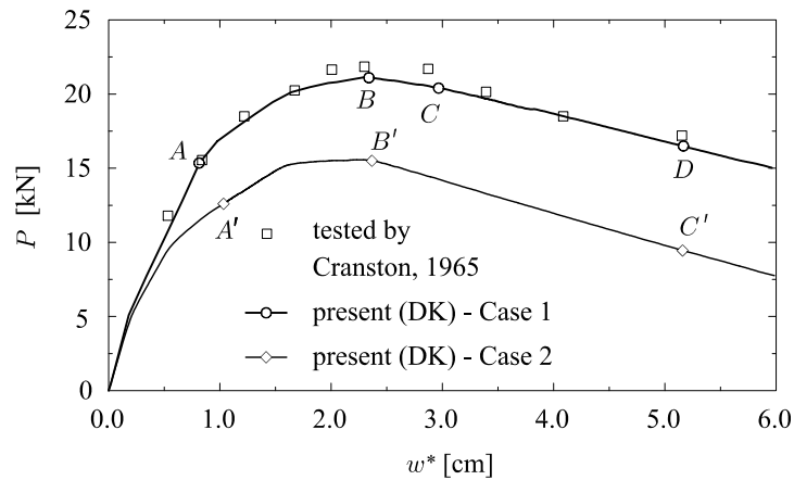
Figure 17. Cranston's portal frame. The load-displacement curve as a function of the reinforcement layout, Case 1 and Case 2.
