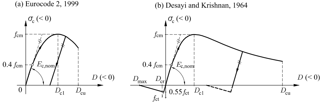
Figure 2: Constitutive laws of concrete according to (a) Eurocode 2 (1999), and (b) Desayi and Krishnan (1964).
