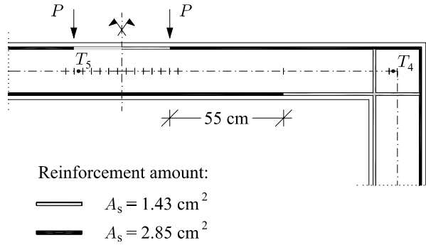
Figure 19. Cranston's portal frame with a geometric imperfection. Finite-element mesh.
