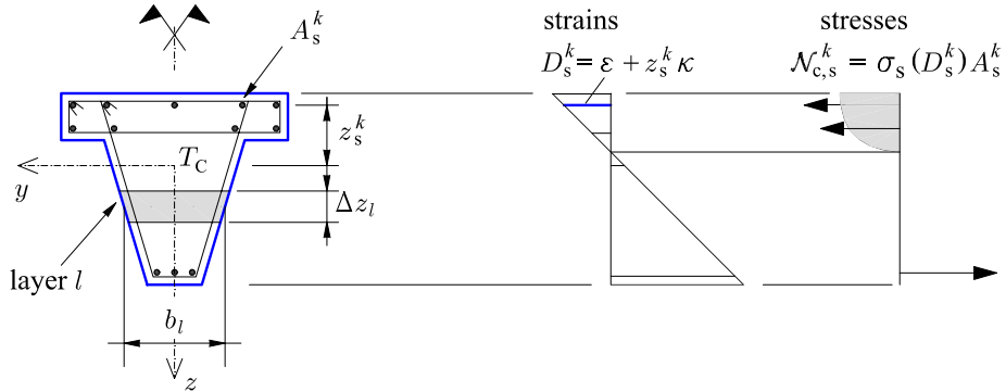
Figure 4: Typical cross-section.
