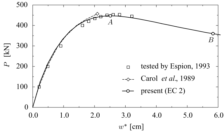
Figure 6. Foure’s column. Loading factor vs lateral deflection curve.
