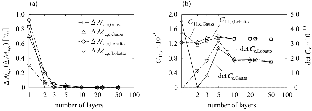
Figure 23. Cranston's portal frame. The accuracy of numerical integrations over the cross-section at T_1 ; P = 20 kN. (a) \Delta \mathcal{N}_{c,c}(\Delta \mathcal{M}_{c,c}) = \left| \frac{\mathcal{N}(\mathcal{M})_c - \mathcal{N}(\mathcal{M})_{c,50}}{\mathcal{N}(\mathcal{M})_{c,50}} \right| in concrete, (b) C_{11,c} in concrete, and \det \mathbf{C}_c of the concrete part of the cross-section.
