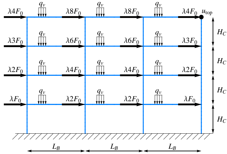
Figure 6.11: Symmetric frame: geometry and loading
