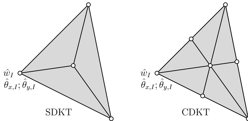
Figure 6.2.1: Subdivision schemes for the DKT element
