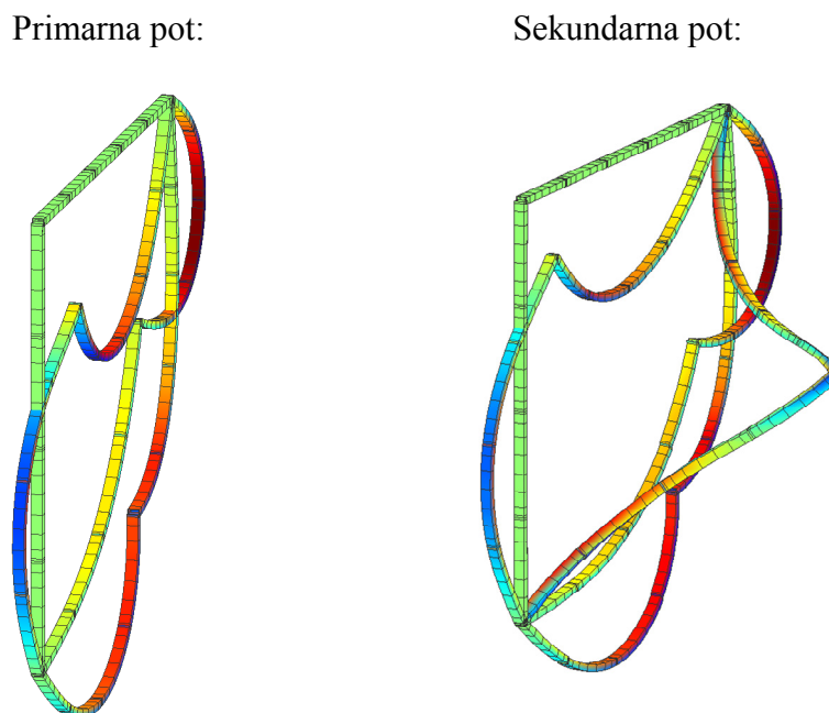
Slika 4.11: Deformirane lege kolenastega nosilca po primarni in sekundarni veji. Figure 4.11: Deformed shapes of right-angle frame for primary and bifurcation path.
