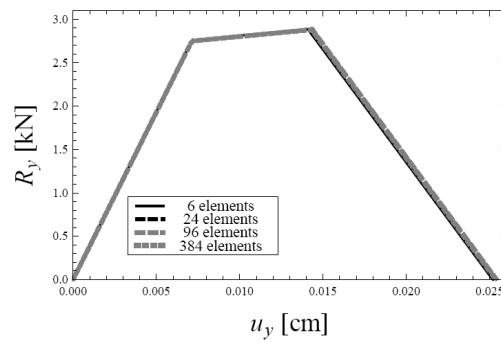
Figure 26: Total reaction force versus imposed displacement curves
