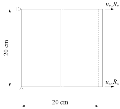
Figure 6: Tension test on a square block
