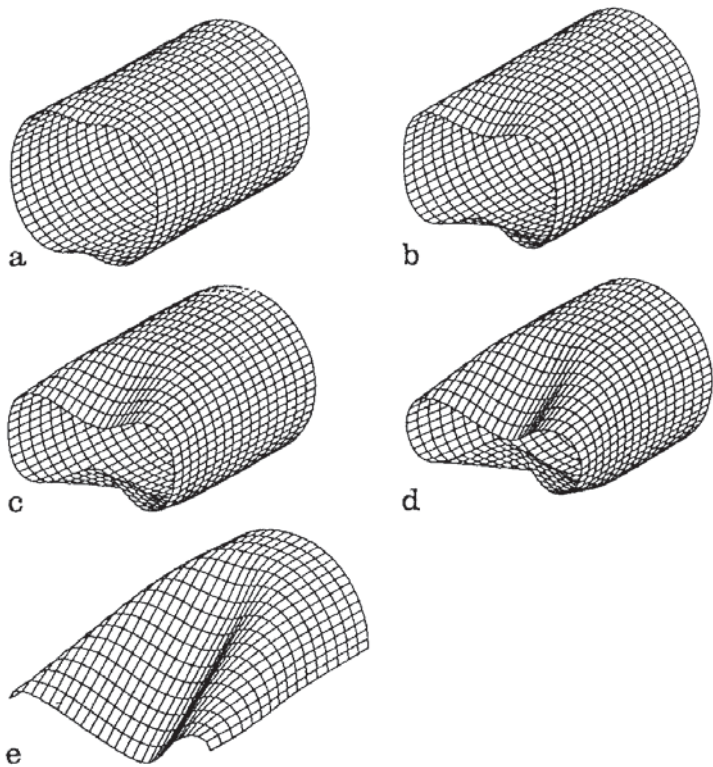
Fig. 14a-e. Clamped cylinder: Deformed configuration of the shell at 5 different load stages. Displacements under the forces are: a R/4 , b R/2 , c 3R/4 , d R and e 1.608R
