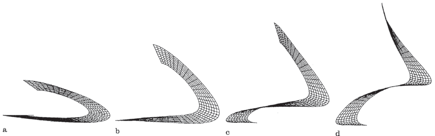
Fig. 21a-d. Ring plate: Deformed finite element mesh ( 8 \times 48 ) at different loading stages: a f = 11.726 , b f = 53.786 , c f = 105.55 , d f = 202.53
