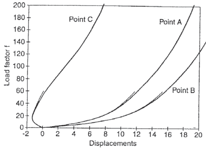
Fig. 20. Ring plate: Load versus displacement curves for points A, B and C
