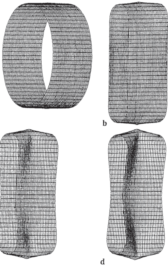
Fig. 18a-d. Cylinder with free ends: Deformed finite element mesh ( 16 \times 16 ) at various stages of loading: a F/F_0 = 0.04 , b F/F_0 = 0.33 , c F/F_0 = 0.60 , d F/F_0 = 1.0
