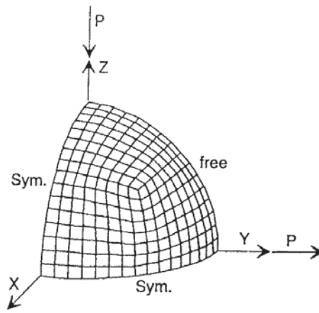
Fig. 8. Hemispherical shell: Geometry and loading
