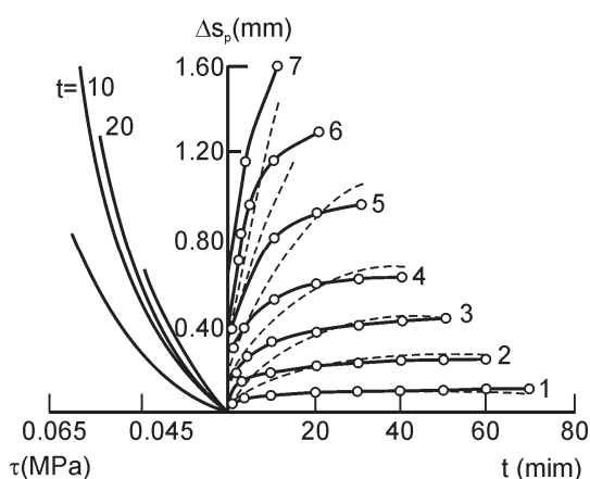
Slika 11.16: Primeri krivulj strižnega lezenja (Meschyran, 2006). Figure 11.16: Examples of shear creep curves (Meschyran, 2006).
