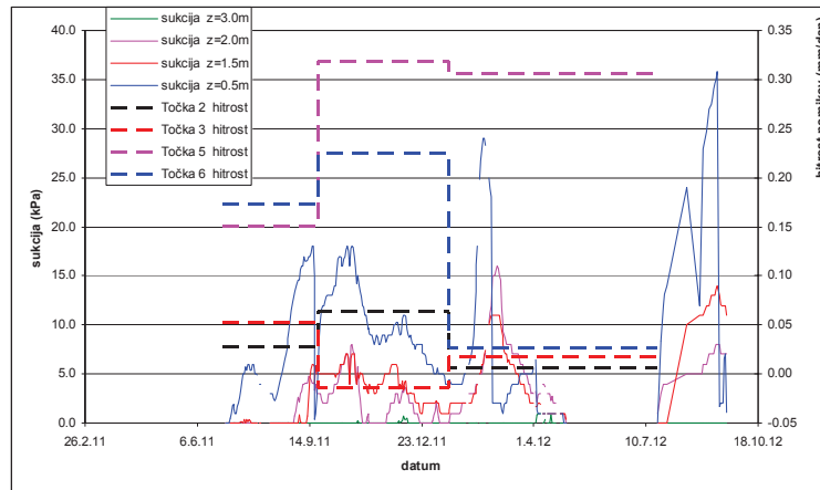
Slika 12.17: Spreminjanje hitrosti lezenja plazu in sukcije s časom. Figure 12.17: Change in creep rate and suction with time.
